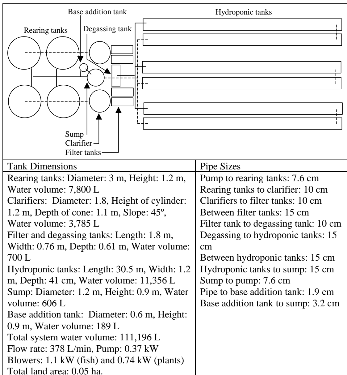
Figure 1. Current design of the UVI commercial aquaponic system (CA2).
